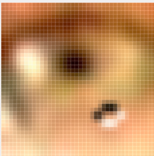
Bilinear
