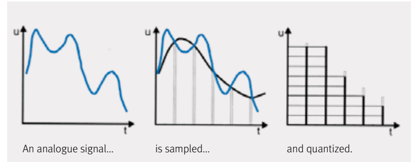
Fig. 8c: If the sampling rate is too low, the reproduction will be poor.
